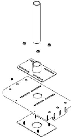
Figure 1. CMA-150 Installation
