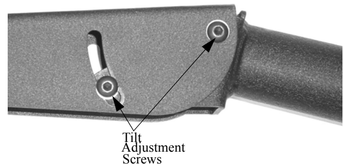
Figure 7. Tilt Adjustment
