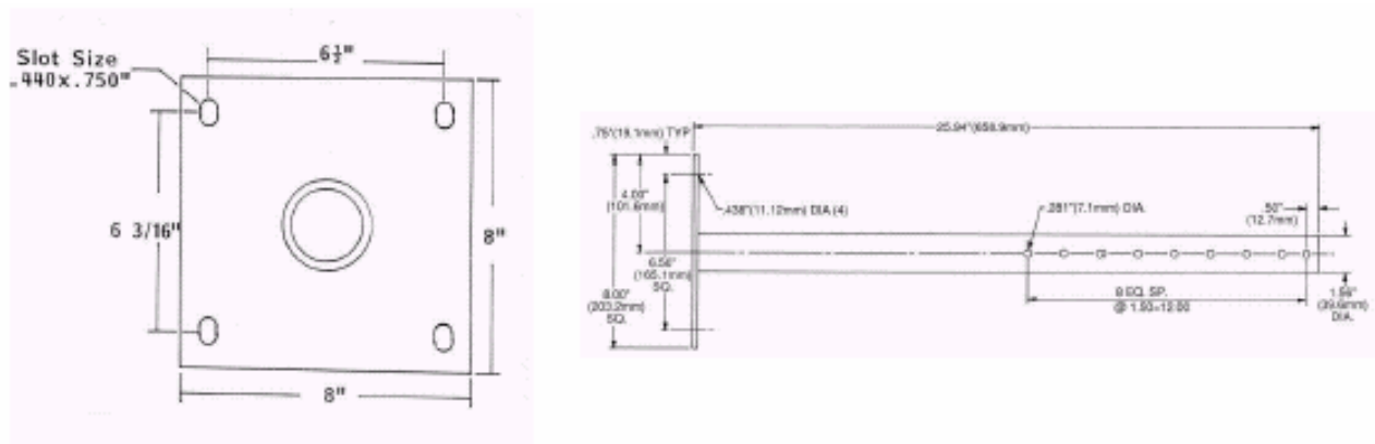
Figure 1. ELE-CP2446 Flat Ceiling Plate with Adjustable Extension Column
