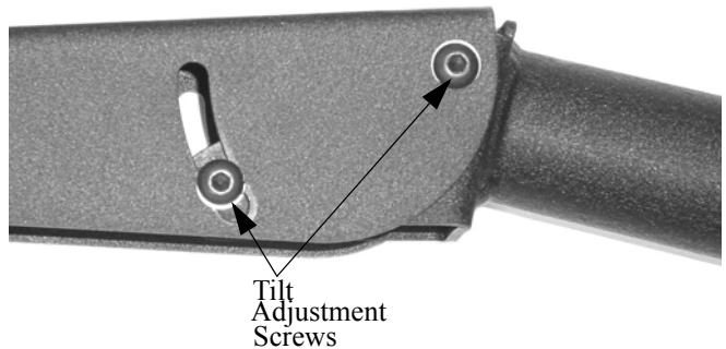
Figure 7. Tilt Adjustment
