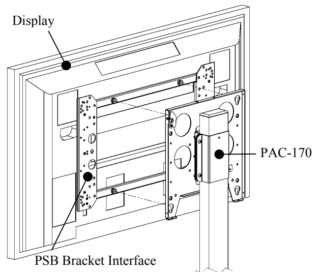
Figure 3. Mount the Display
