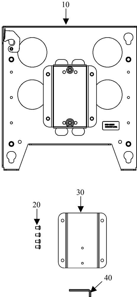
Figure 1. Parts
