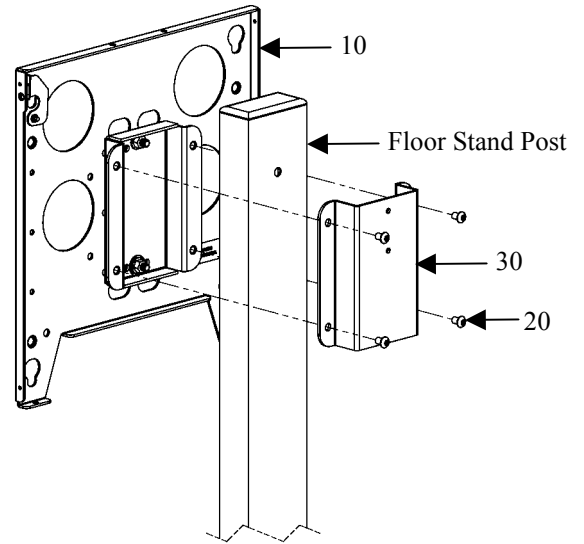
Figure 2. Attach PAC-170 to Floor Stand
