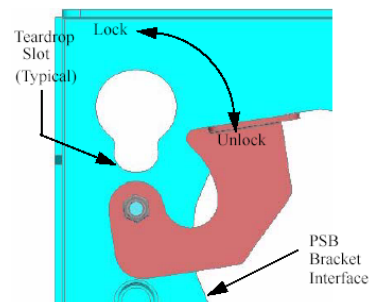
Figure 4. Locking Device
