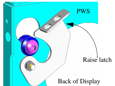
FIGURE 3. RAISE LATCH
