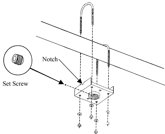
Figure 1 - Ceiling Plate Assembly
