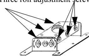
Figure 10. Roll Adjustment
