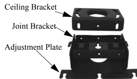
Figure 7. RPA Disassembly
