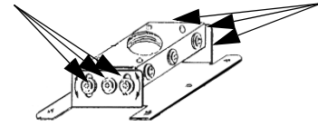
Figure 9. Adjust Pitch
