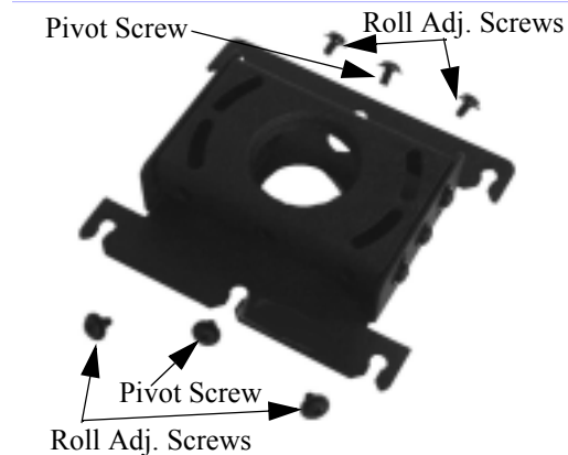
Figure 6. RPA Screws
