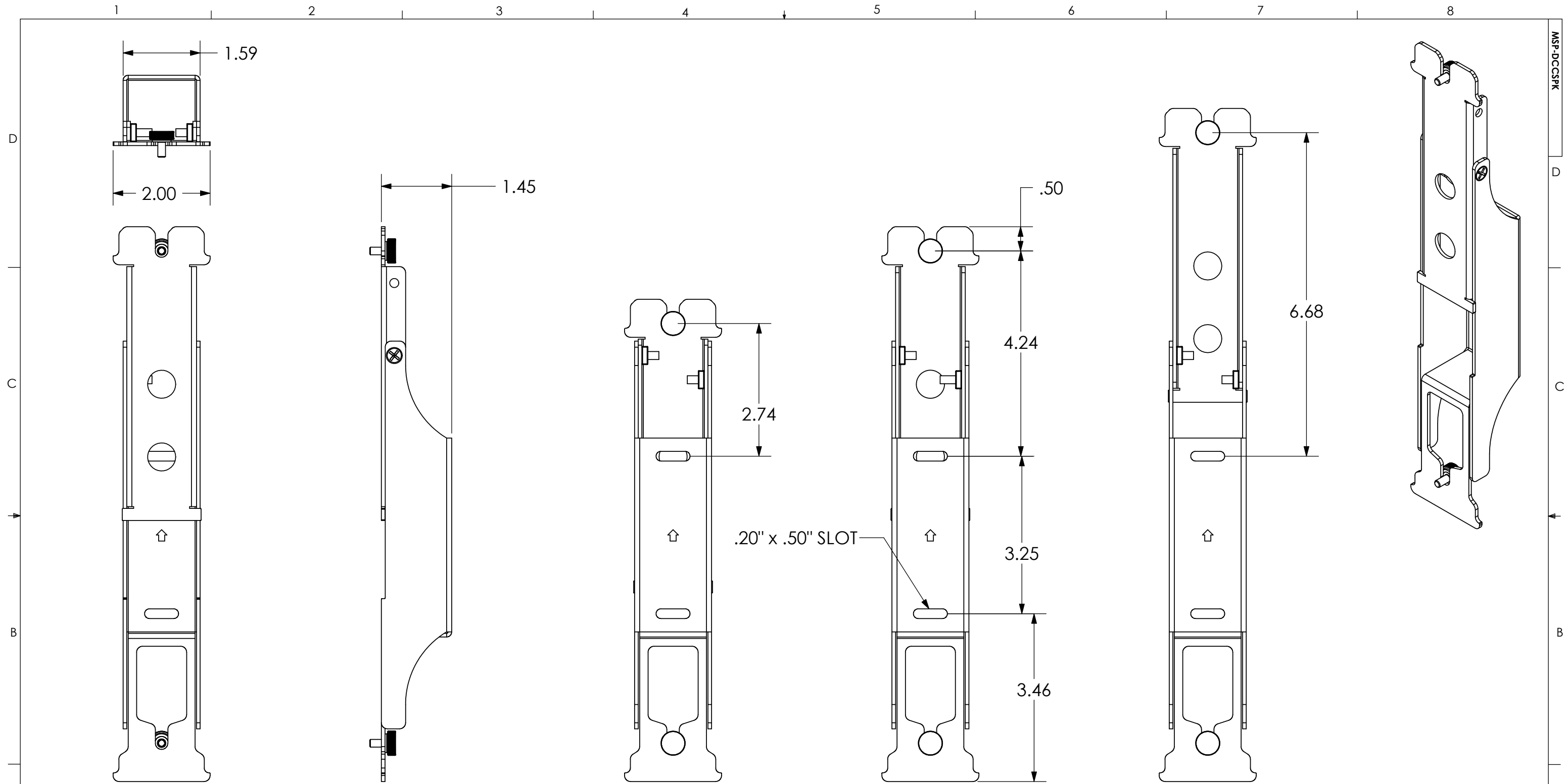
37" DISPLAY SPEAKERS
