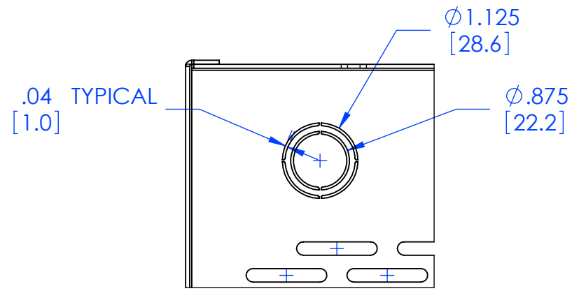
DETAIL A SCALE 1 : 2 (KNOCKOUT)
