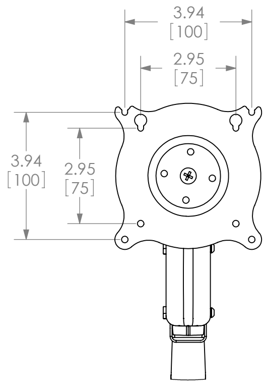
DETAIL A SCALE 1 : 3
