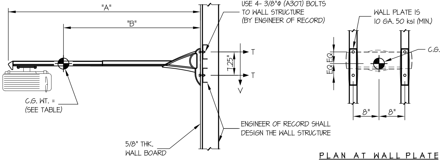
PLAN AT WALL PLATE
